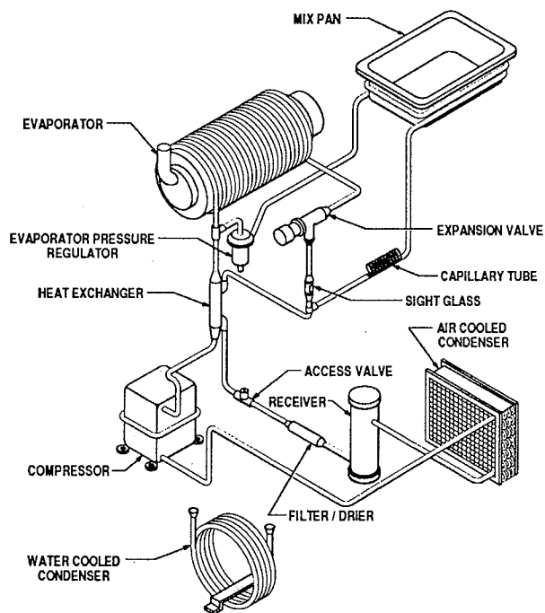
Refrigeration System
