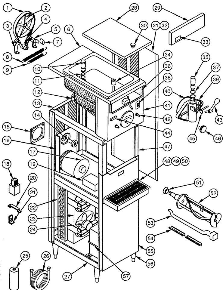
Exploded View
