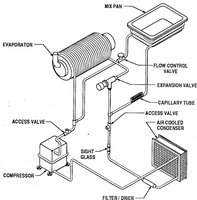
Refrigeration System
