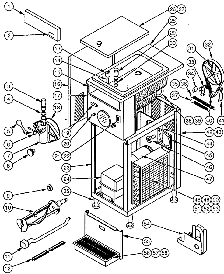
Exploded View
