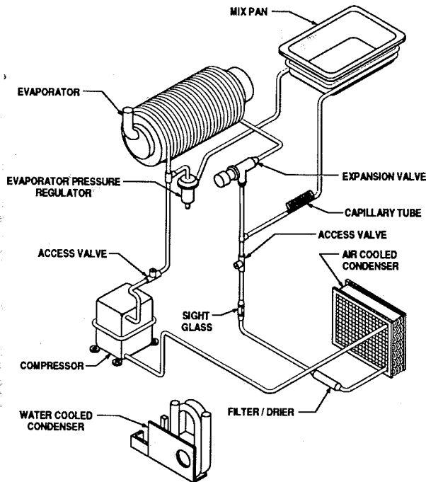
Refrigeration System
