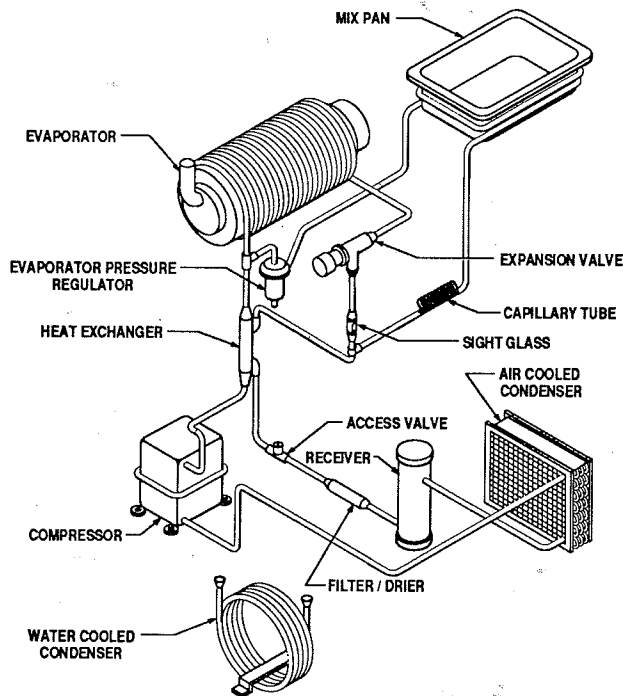
Refrigeration System
