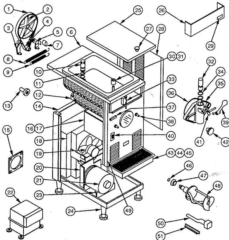
Exploded View
