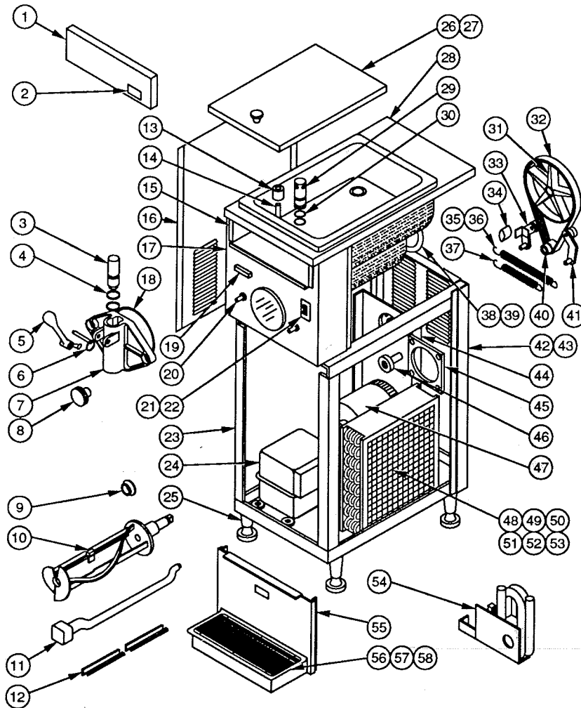
Exploded View
