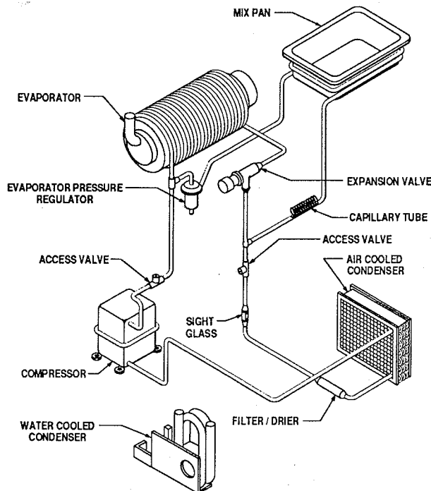
Refrigeration System
